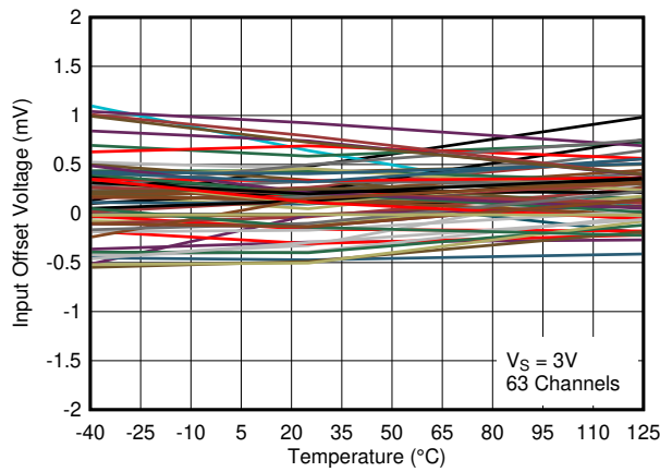
图 7-7. Input Offset Voltage vs. Temperature at 3V
