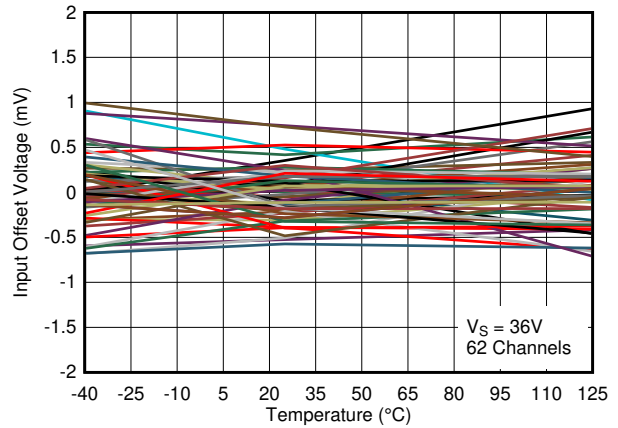
图 7-10. Input Offset Voltage vs. Temperature at 36V
