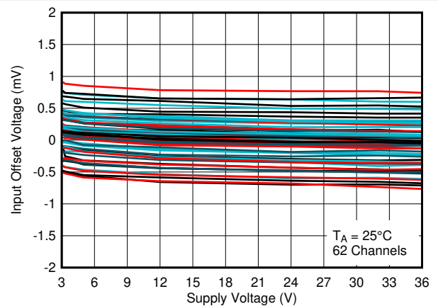
图 7-12. Input Offset Voltage vs. Supply Voltage at 25^\circ\text{C}
