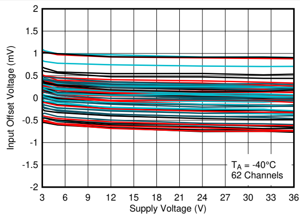
图 7-11. Input Offset Voltage vs. Supply Voltage at -40^\circ\text{C}
