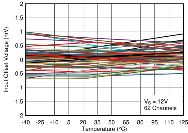
图 7-9. Input Offset Voltage vs. Temperature at 12V
