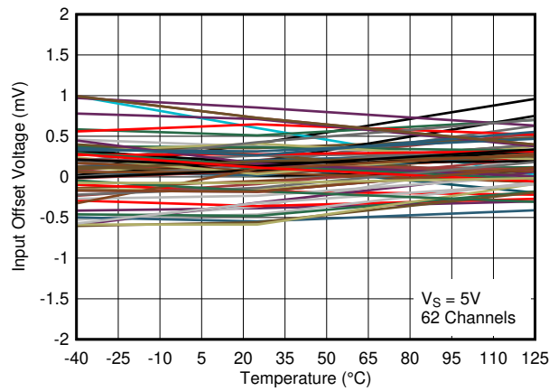
图 7-8. Input Offset Voltage vs. Temperature at 5V
