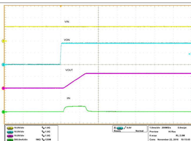
Figure 29. TPS22810 Inrush Current with C_L = 22 \mu F , CT = 4700 pF
