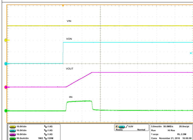
Figure 28. TPS22810 Inrush Current With C_L = 22 \mu F , CT = 0 pF
